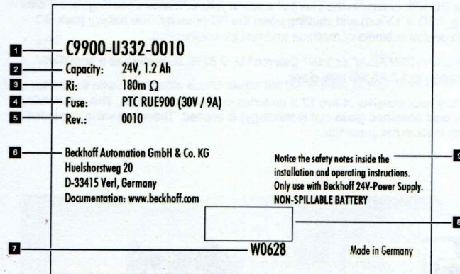
Fig. 2: C9900-U332_name plate
